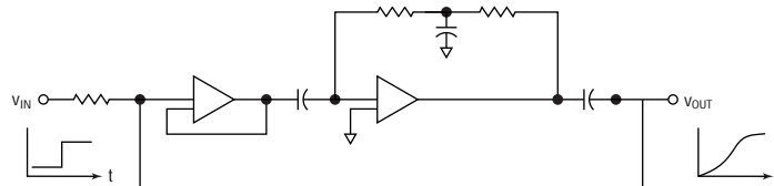
Figure 20 Analog Filter
