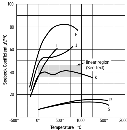
Figure 17 Seebeck Coefficient vs. Temperature
