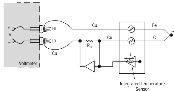
Figure 15 Practical Hardware Compensation
