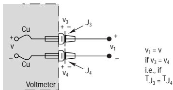
Figure 7 Junction Voltage Cancellation
