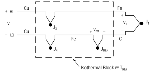
Figure 9b Joining the Isothermal Blocks
