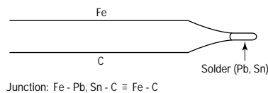
Figure 25 Soldering a Thermocouple
