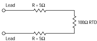
Figure 38 Effect of Lead Resistance
