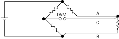
Figure 41 3-Wire Bridge
