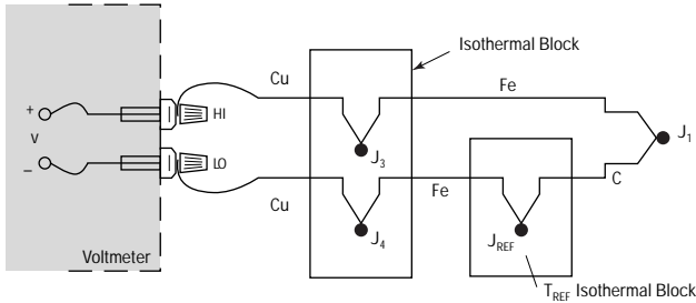
Figure 9a Eliminating the Ice Bath
