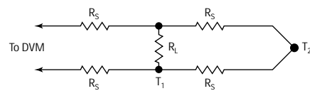
Figure 28 Virtual Junction
