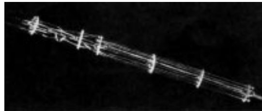
Figure 36 Bird-Caged PRTD
