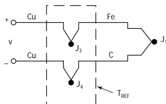
Figure 11 Equivalent Circuit
