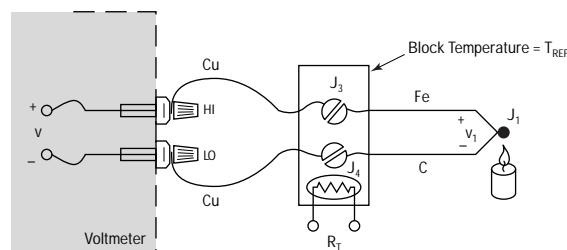
Figure 12 External Reference Junction - No Ice Bath
