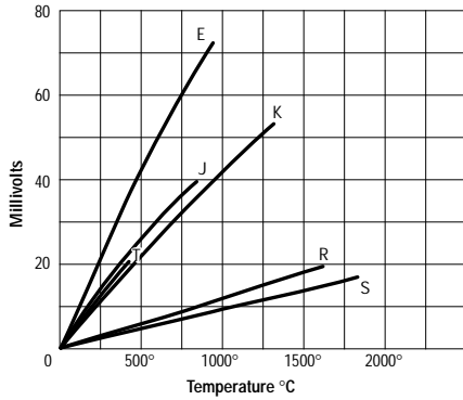
Figure 16 Thermocouple Temperature vs. Voltage Graph
