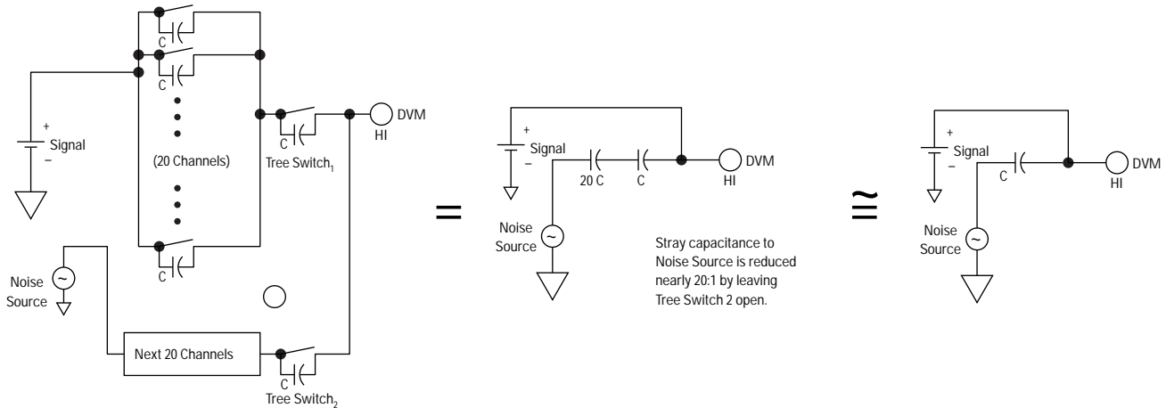
Figure 19 Tree Switching
