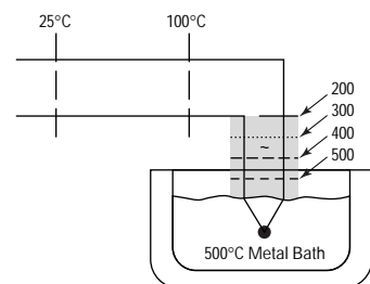
Figure 26 Gradient Produces Voltage
