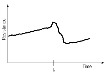
Figure 32 Thermocouple Resistance vs. Time
