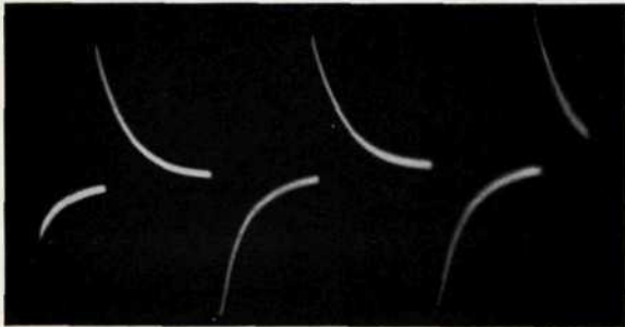
Square Wave Distortion from poor low-frequency response. (Phase shift of low frequency components which always accompanies cut-off.)
