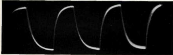
Square Wave Distortion from poor high frequency response.
