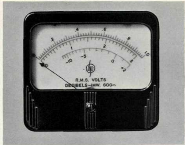
Voltmeter Face. Note both voltage and D. B. calibrations.
