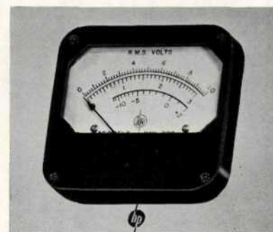
Meter face on 400A. Note both voltage and D. B. calibrations.
