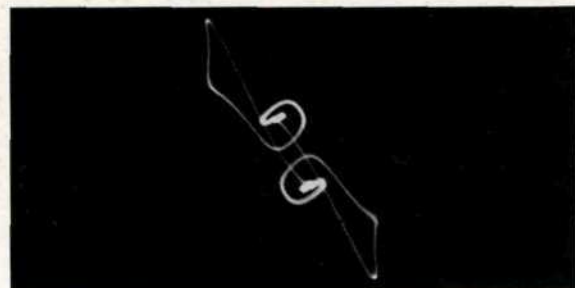
Same as left. One amplifier defective shows up immediately whereas without square wave a long point by point frequency response would be required to discover deviation from standard.
