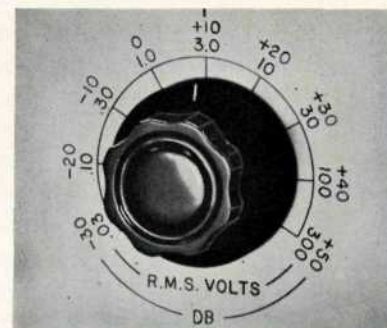
Range selection switch on 400A. Note both voltage and D. B. calibrations.
