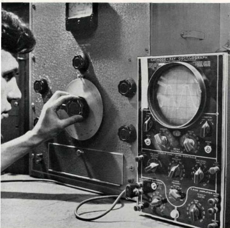
Here a Model 300A Harmonic Wave Analyzer is being used to measure the distortion components in the output wave of an oscillator.
