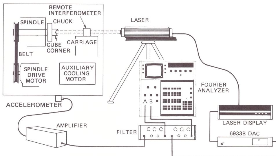
FIGURE 8. Block Diagram for Measurement of Transfer and Coherence Functions
