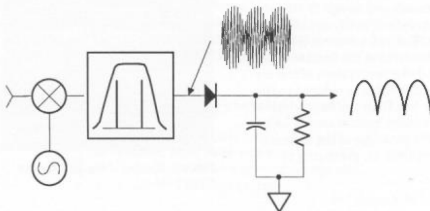
Fig. 23. Output of the envelope detector follows the peaks of the IF signal.
