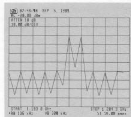
Fig. 39. Rosenfell when signal peak falls between data points (fewer trace points exaggerate the effect).
