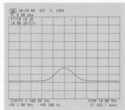
Fig. 25. Display of Fig. 24 after full smoothing.
