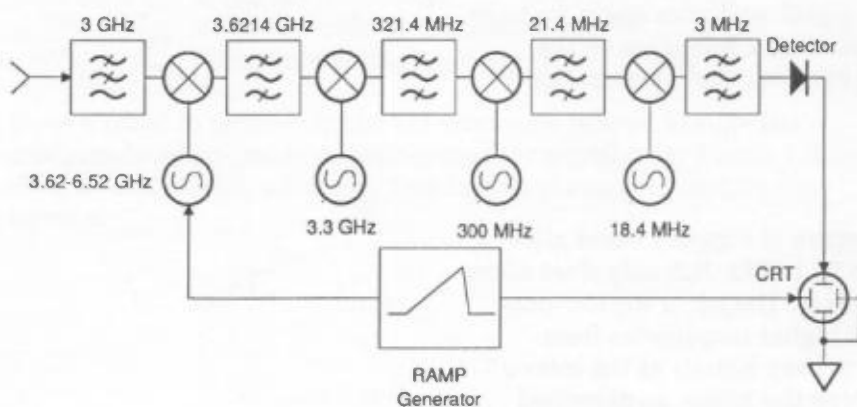
Fig. 10. Most spectrum analyzers use two to four mixing steps to reach the final IF.
