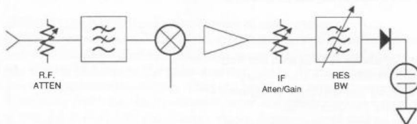
Fig. 40. Controls that affect amplitude accuracy.
