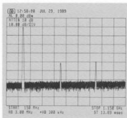
Fig. 3. Harmonic distortion test.
