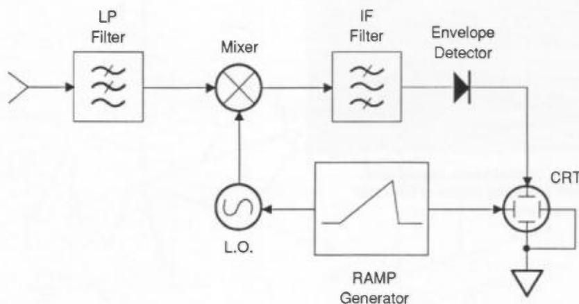
Fig. 7. Superheterodyne spectrum analyzer.
