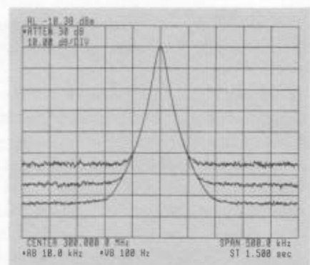
Fig. 42. Other analyzers keep reference level constant by changing IF gain, so as RF attenuator is changed, the analyzer's noise moves, but an input signal does not.
