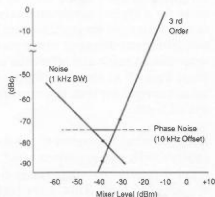
Fig. 53. Phase noise can limit third-order intermodulation tests.
