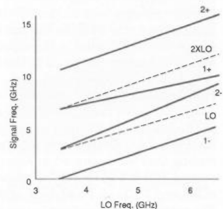
Fig. 59. Signals in the 1- frequency range produce single, unambiguous responses in the low-band, high-IF case.
