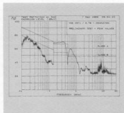
Fig. 6. Conducted emissions plotted against VDE limits as part of EMI test.
