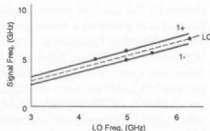
Fig. 60. Tuning curves for fundamental mixing in the high-band, low-IF case.
