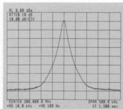
Fig. 8. Typical spectrum analyzer display with control settings.
