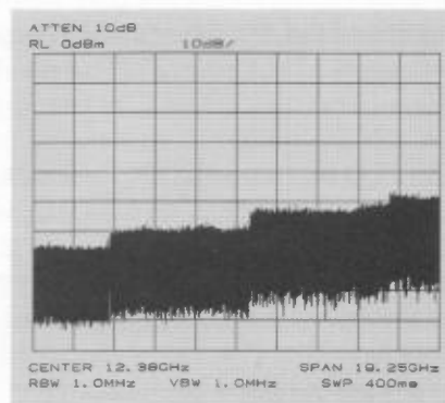
Fig. 63. Steps in the noise floor indicate changes in sensitivity with changes in LO harmonic used in the mixing process.
