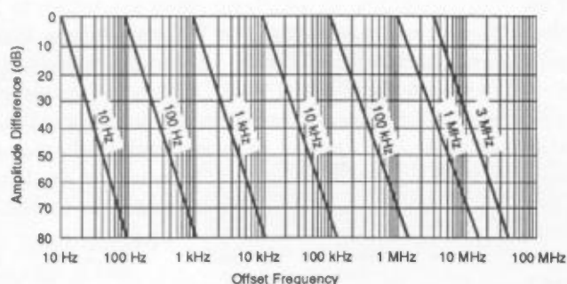
Fig. 16. Resolution versus offset for HP 8566B.
