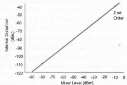
Fig. 68. Extended second-order distortion graph.
