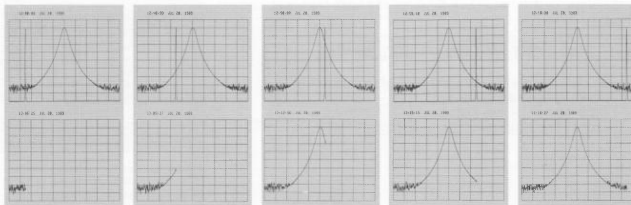
Fig. 11. As a mixing product sweeps past the IF filter, the filter shape is traced on the display.
