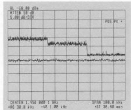
Fig. 27. On analyzers using pos peak display mode, reducing the video bandwidth lowers the peak noise but not the average noise. Lower trace shows average noise.
