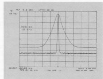
Fig. 43. Displayed noise level changes as 10 \cdot \log(BW_2/BW_1) .
