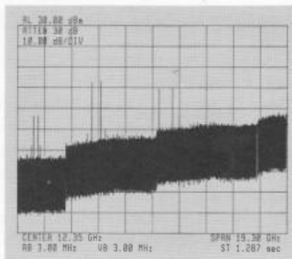
Fig. 70. Preselection makes wide spans practical.
