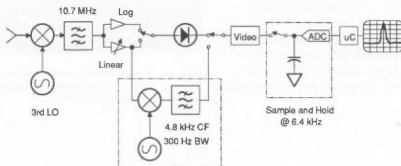
Fig. 17. Digital implementation of 10, 30, and 100 Hz resolution filters in HP 8560A, 8561B, and 8563A.
