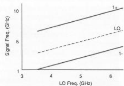
Fig. 58. Tuning curves for fundamental mixing in the low-band, high-IF case.
