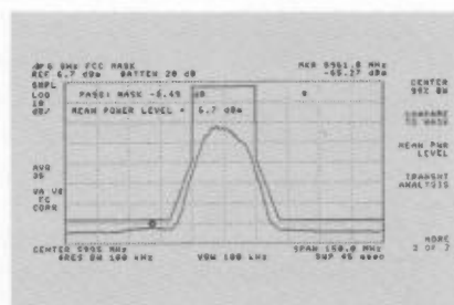
Fig. 5. Digital radio signal and mask showing limits of spectral occupancy.
