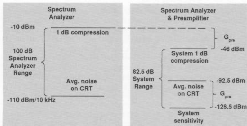
Fig. 45. If the displayed noise goes up when a preamplifier is connected, measurement range is diminished by the amount the noise changes.
