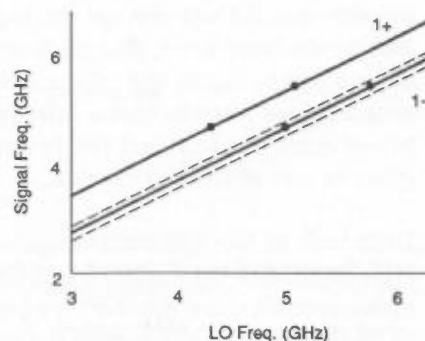
Fig. 66. A preselector allows a signal to reach the mixer only when the analyzer is tuned to receive the signal.
