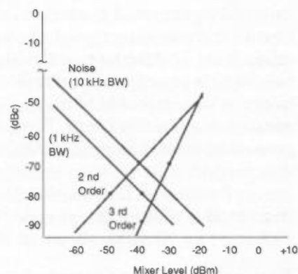
Fig. 52. Reducing resolution bandwidth improves dynamic range.
