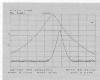
Fig. 13. A low-level signal can be lost under skirt of the response to a larger signal.
