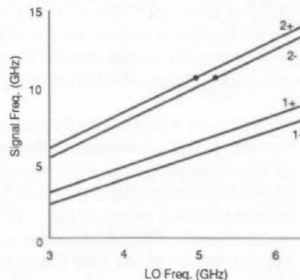
Fig. 65. A response at a given LO frequency does not uniquely determine signal frequency.
