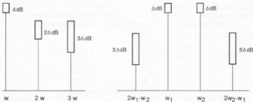
Fig. 50. Changing the level of fundamental tone ( w ) or tones ( w_1 , w_2 ) at the mixer affects internally generated distortion.
