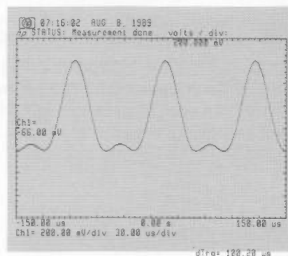
Fig.1. Complex time-domain signal.
