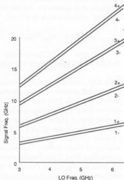
Fig. 61. Tuning curves for n = 1 through 4 in the high-band, low-IF case.
