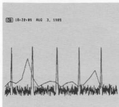
Fig. 34. The actual comb and results of the sample display mode over a 500-MHz span. When resolution bandwidth is narrower than the sample interval, the sample mode can give erroneous results. (The sample trace has only 20 points to exaggerate the effect.)
