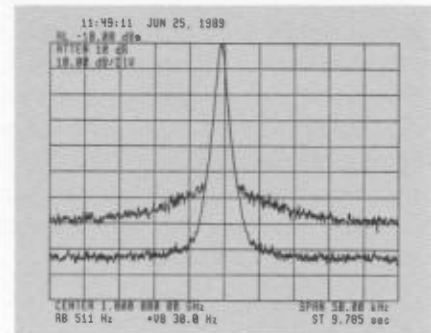
Fig. 64. Difference in phase noise between fundamental and fourth-harmonic mixing.
