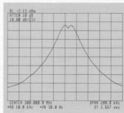
Fig. 12. Two equal-amplitude sinusoids separated by the 3 dB BW of the selected IF filter can be resolved.
