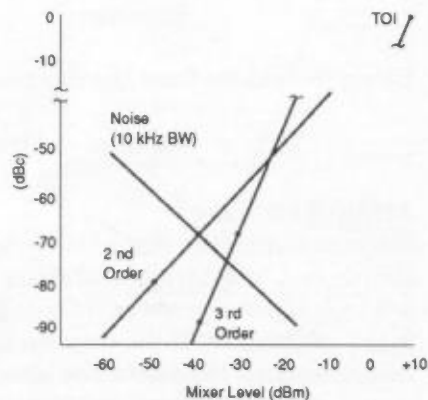
Fig. 51. Dynamic range versus distortion and noise.
