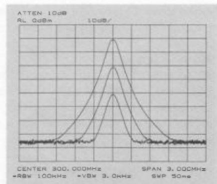
Fig. 41. Some spectrum analyzers change reference level when RF attenuator is changed, so an input signal moves on the display, but the analyzer's noise does not.
