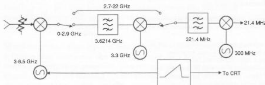
Fig. 57. Switching arrangement to provide a high IF for the low band and a low IF for the high bands.
