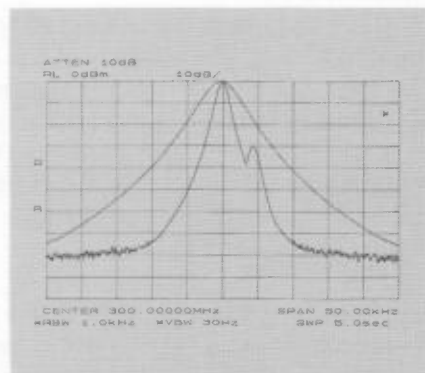
Fig. 15. The 3 kHz filter does not resolve smaller signal, the 1 kHz filter does.
