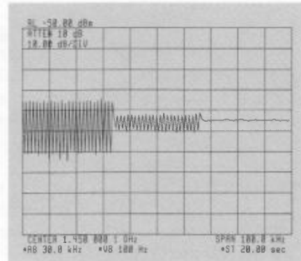
Fig. 26. Smoothing effect of video-resolution bandwidth ratios of 3, 1/10, and 1/100 (on a single sweep).
