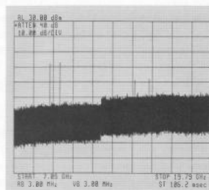
Fig. 62. The number of responses is a function of signal frequency and analyzer span.
