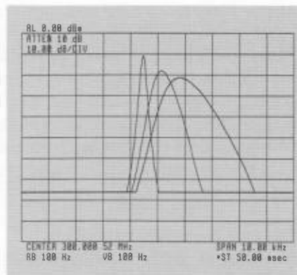
Fig. 21. Sweeping an analyzer too fast causes a drop in displayed amplitude and a shift in indicated frequency.
