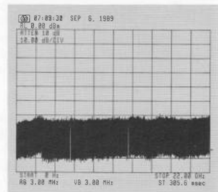
Fig. 72. Fundamental mixing across the entire tuning range gives the HP 71210 the same sensitivity at 22 GHz as at 1 GHz.
