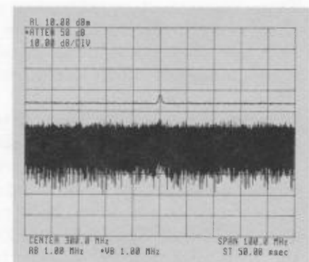
Fig. 44. Video filtering makes low-level signals more discernable. (The average trace was offset for visibility.)
