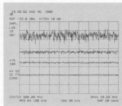
Fig. 28. Effect of video (digital) averaging for 1, 5, 20, and 100 sweeps (top to bottom).
