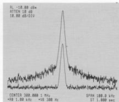
Fig. 19. Phase noise is displayed only when a signal is displayed far enough above the system noise floor.
