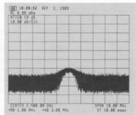
Fig. 24. Spectrum analyzers display signal plus noise.
