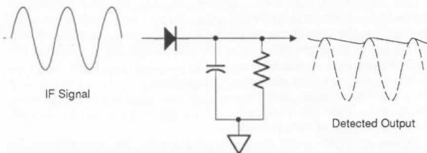
Fig. 22. Envelope detector.
