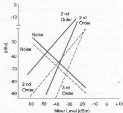
Fig. 55. Dynamic range for 1.5-dB maximum error.
