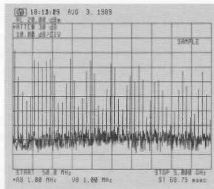
Fig. 33. A 5-GHz span of a 100-MHz comb in the sample display mode. The actual comb values are relatively constant over this range.
