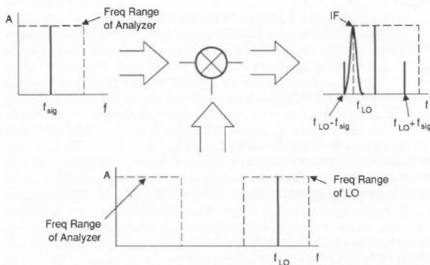
Fig. 9. The LO must be tuned to f_{IF} + f_{sig} to produce a response on the display.
