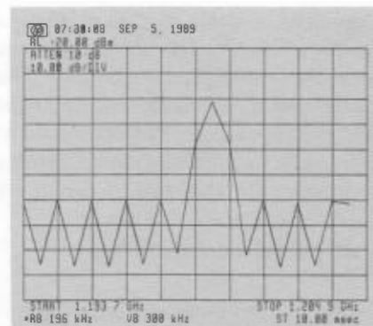
Fig. 38. When detected signal only rises or falls, as when mixing product sweeps past resolution filter, rosenfell displays maximum values.
