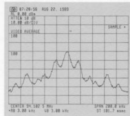
Fig. 29. Video (analog) filtering and video (digital) averaging yield different results on an FM broadcast signal.
