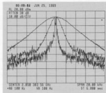
Fig. 18. LO residual FM is seen only when the resolution bandwidth is less than the peak-to-peak FM.
