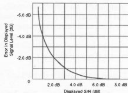
Fig. 56. Error in displayed signal amplitude due to noise.
