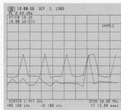
Fig. 36. Comparison of sample and pos peak display modes.
