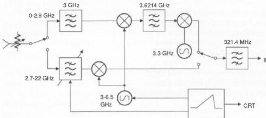
Fig. 67. Front-end architecture of a typical preselected spectrum analyzer.
