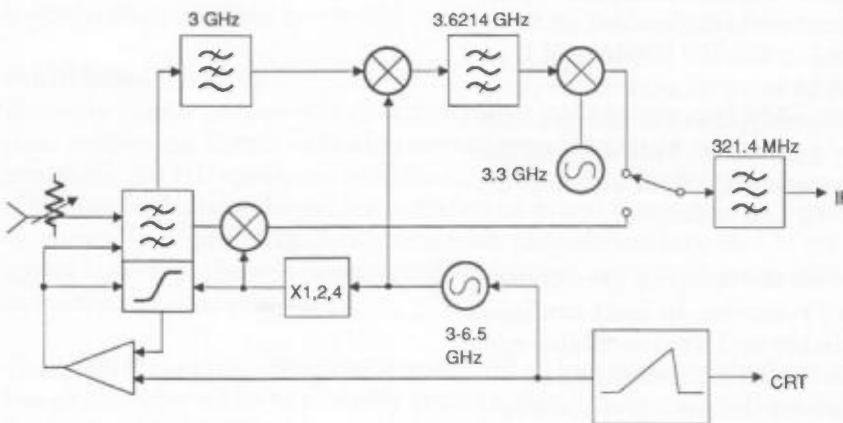
Fig. 71. Front-end architecture of the HP 71210 with solid-state band switch, fundamental mixing to 22 GHz, and dynamic preselector peaking.
