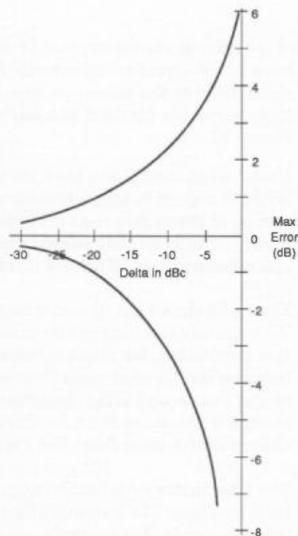
Fig. 54. Uncertainty versus difference in amplitude between two sinusoids at the same frequency.
