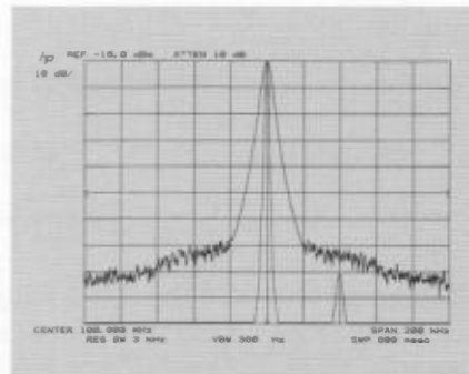
Fig. 20. Phase noise can prevent resolution of unequal signals.
