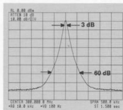
Fig. 14. Bandwidth selectivity, ratio of 60 dB to 3 dB bandwidths, helps determine resolving power for unequal sinusoids.
