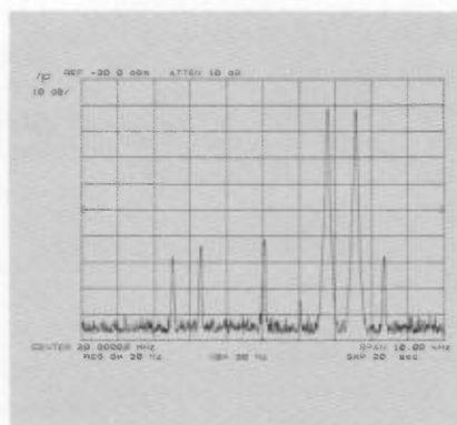
Fig. 4. Two-tone test on SSB transmitter.
