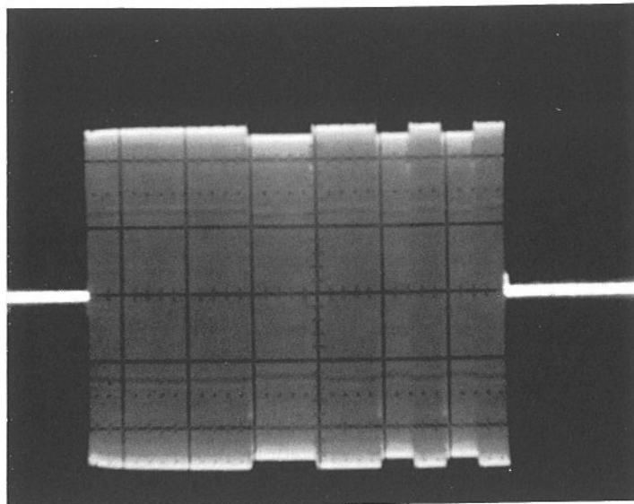
Figure 58. Barker Coded IF Signal
