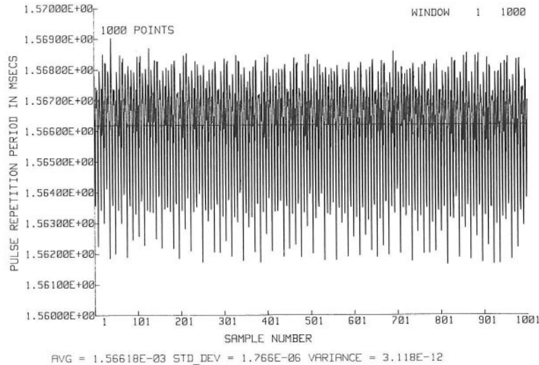
Figure 25. SPS-10 Radar Pulse Repetition Period (1000 Points)
