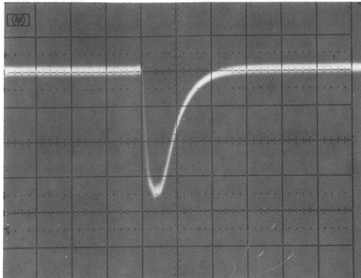
Figure 15. SPS-10E Detected RF Pulse (Short Pulsewidth)
