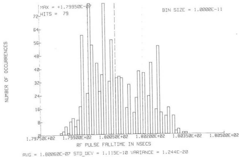
Figure 54. SPS-65(V)1 Radar RF Pulse Falltime Histogram
