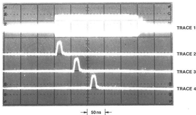
Figure 17. The scope photo shows an RF pulse and multiple exposures on the HP 5345A GATE OUT signal. The 20 ns gate is "walked" through the burst in 50 ns steps.
