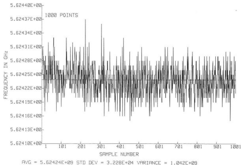
Figure 18. SPS-10 Radar Frequency Point Plot (1000 Points)
