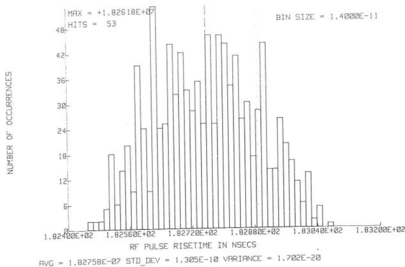
Figure 53. SPS-65(V)1 Radar RF Pulse Risetime Histogram
