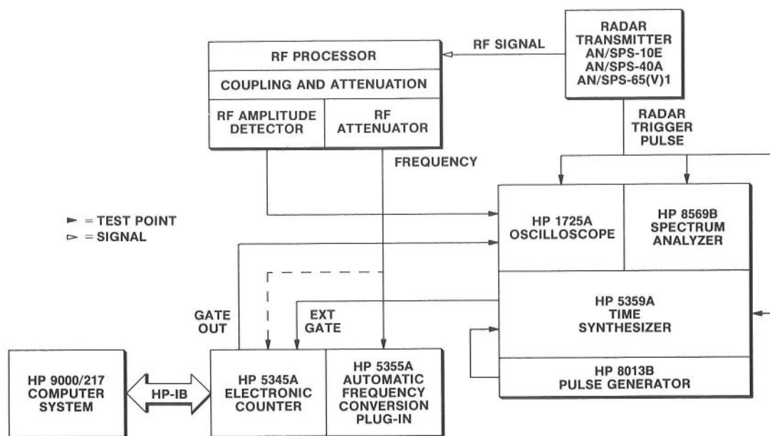
Figure 14. Simplified Block Diagram for Measuring Radar Waveform Average Frequency Profile
