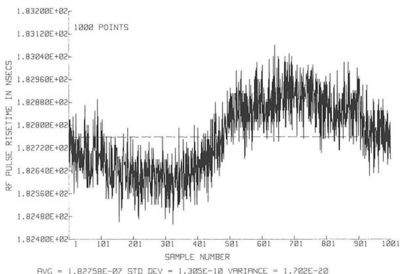
Figure 51. SPS-65(V)1 Radar RF Pulse Risettime
