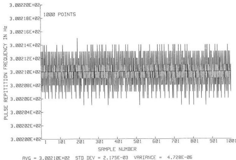
Figure 41. SPS-40A Pulse Repetition Frequency Point Plot
