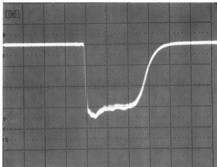
Figure 16. SPS-10E Detected RF Pulse (Long Pulsewidth)
