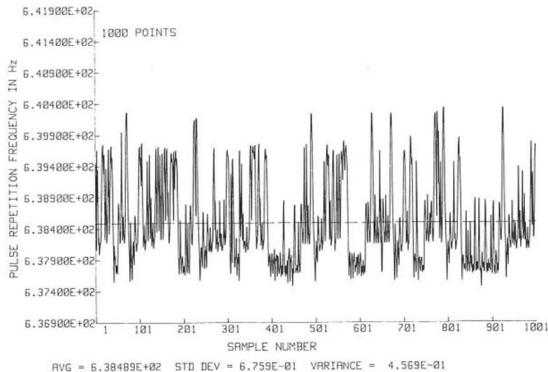
Figure 28. SPS-10 Radar Pulse Repetition Frequency
