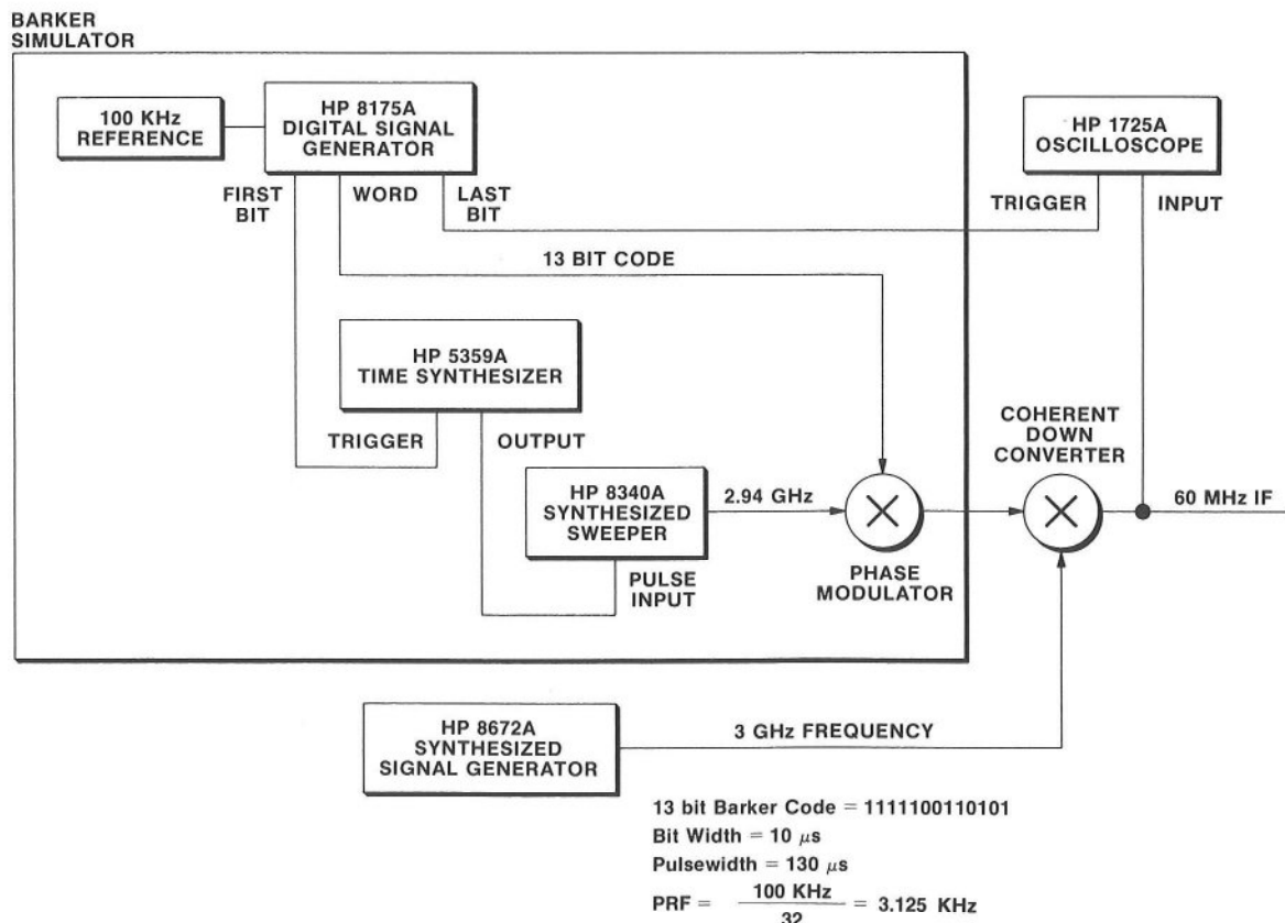
Figure 57. Barker Coded Simulator Generator and Down Converter Block Diagram
