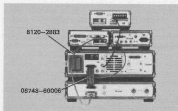
Figure 5. Rear Panel Programming Connections.
