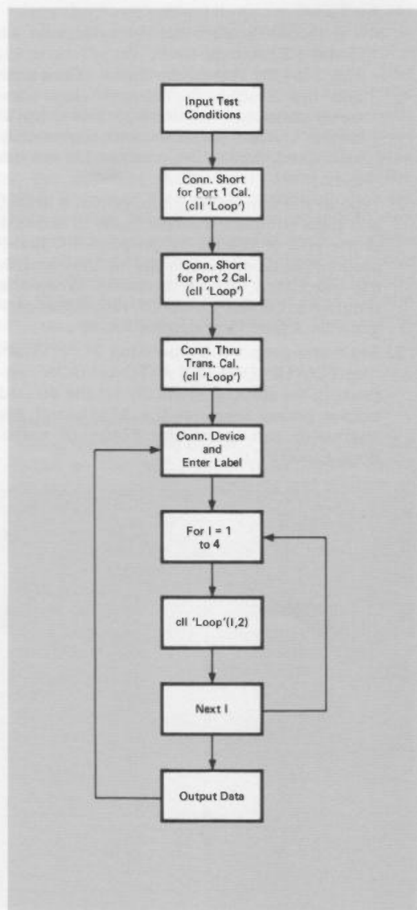
Figure 11. Flowchart of Main Program.
