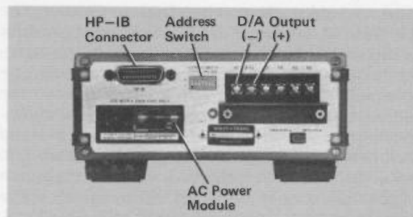
Figure 6. 59501A Rear Panel.
