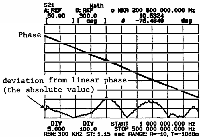
(B) The Deviation from Linear Phase
