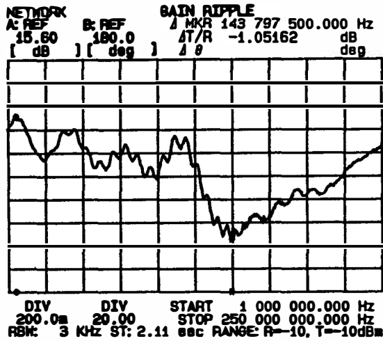
Figure 4. The Gain Ripple
