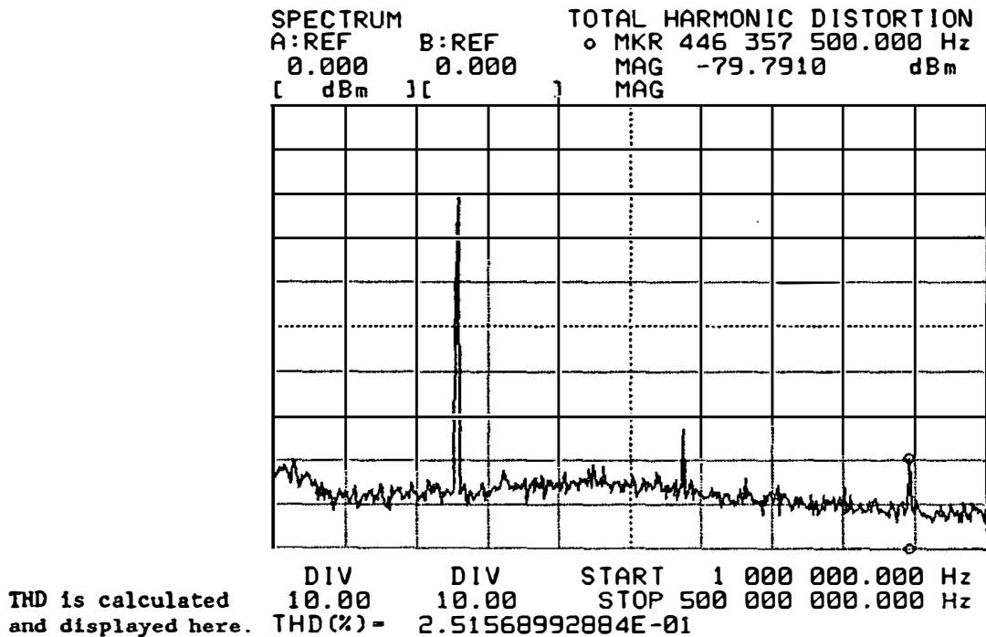
Figure 6. The Total Harmonic Distortion
