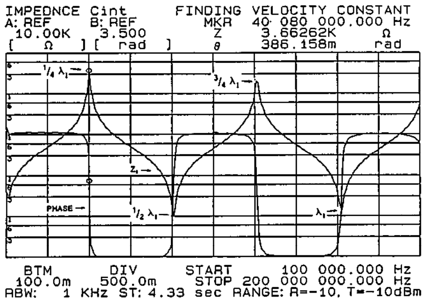
Figure 13. Finding f_1
