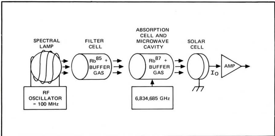
Figure 2-3. RVFR Assembly Block Diagram
