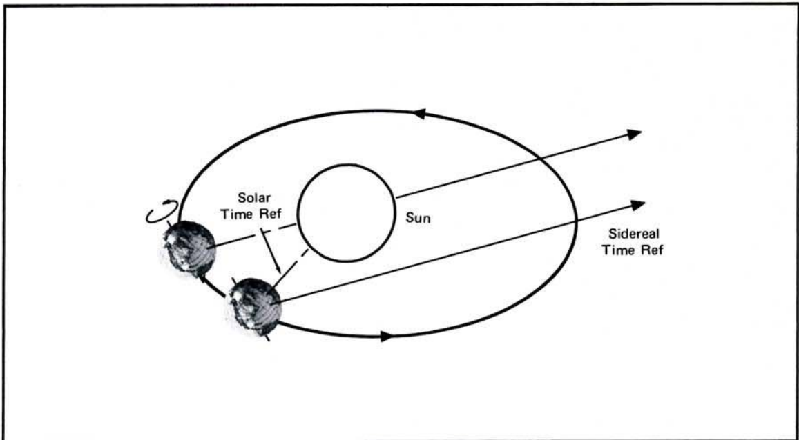
Figure AI-4. Since the length of the solar day is referenced to the sun, orbital motion lengthens the solar day over what it would be if the earth were fixed in position.
