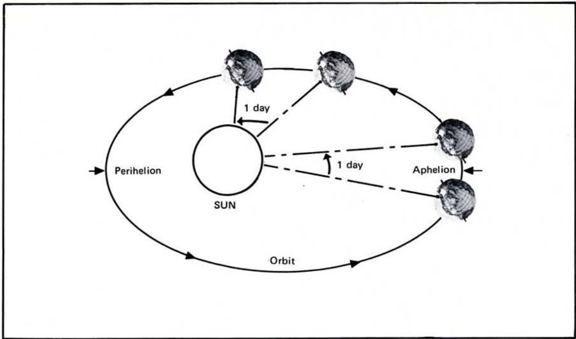
Figure AI-1. Earth's Orbital Motion Exaggerated to Show Varying Effects on Apparent-Solar-Day
