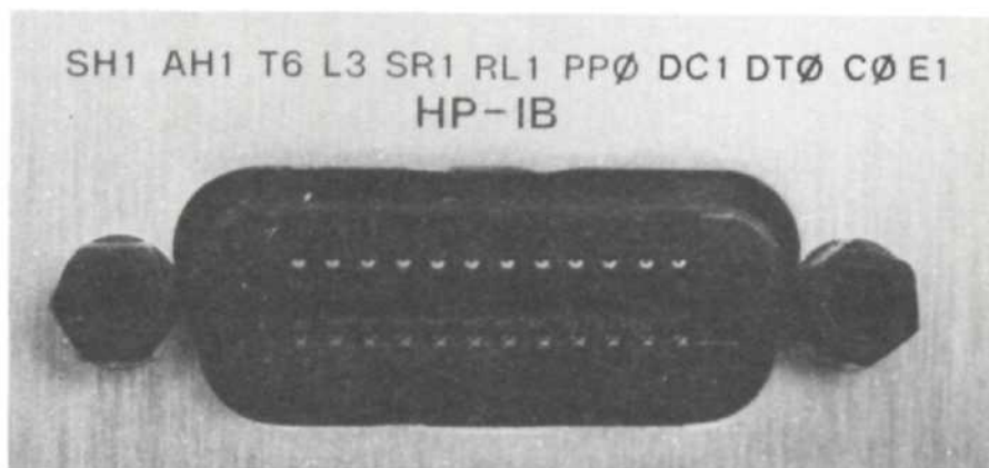
Rear Panel of HP-IB Instrument Showing Interface Capability Codes
